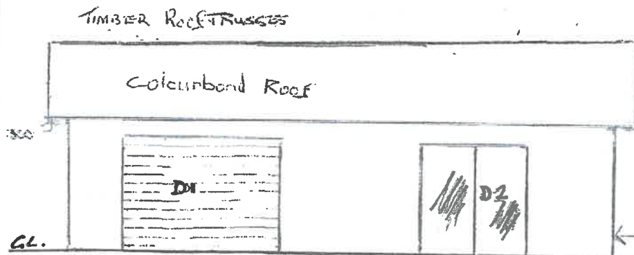
North Elevation
