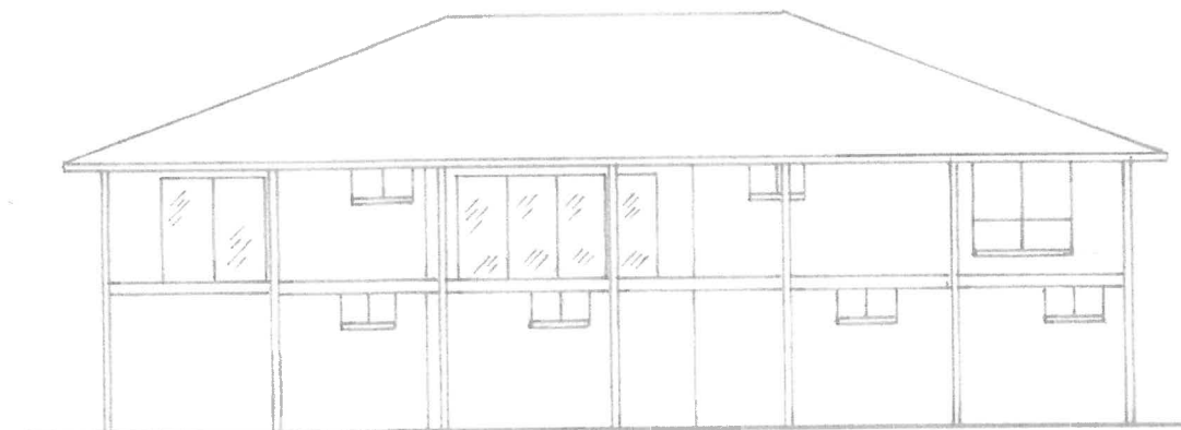
SOUTH ELEVATION
