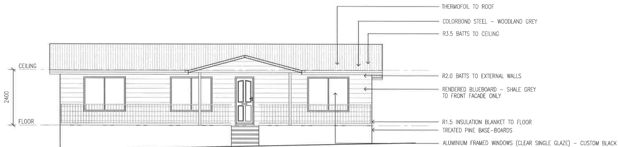
NORTH ELEVATION
