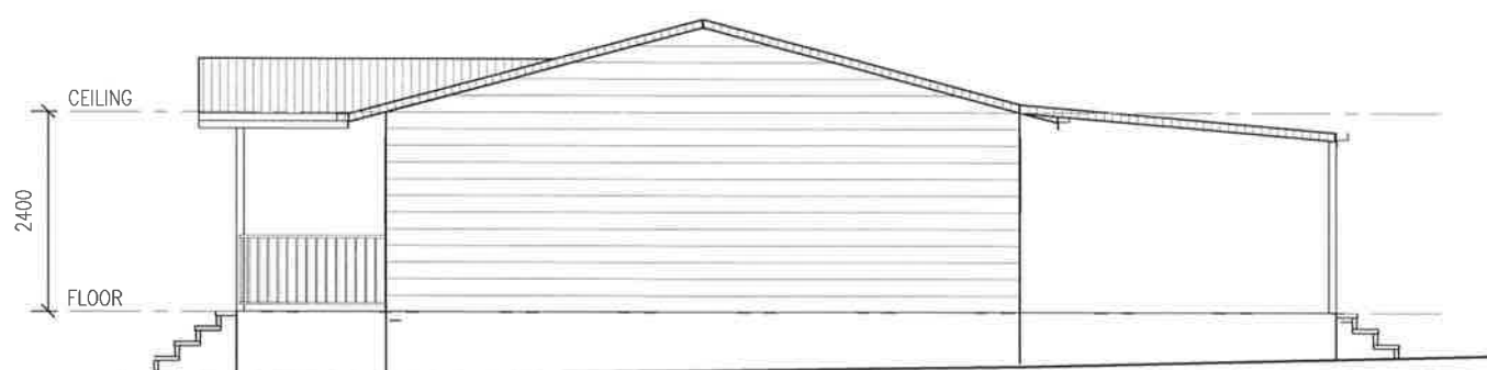
WEST ELEVATION
