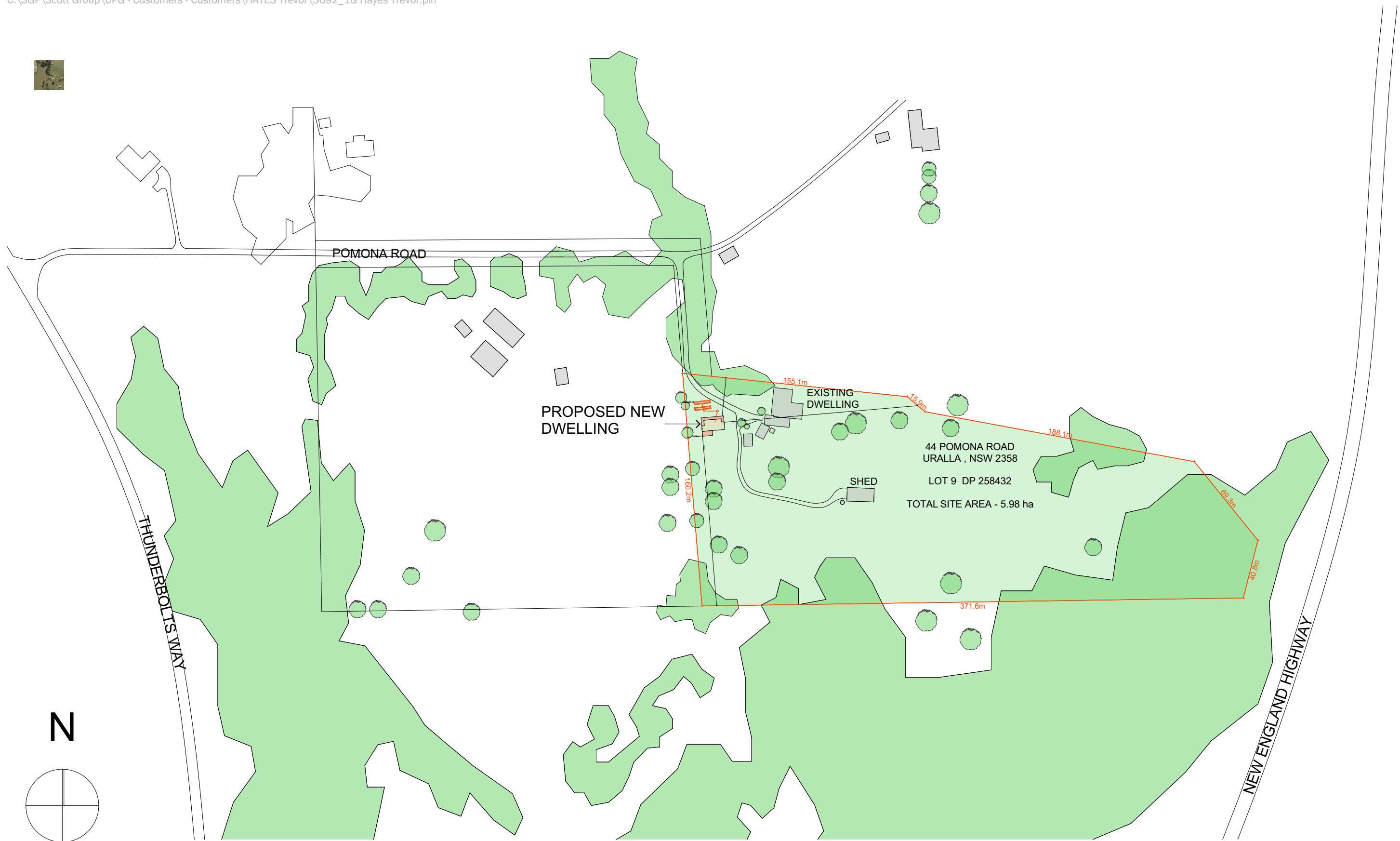
1. locality plan 1:2500
