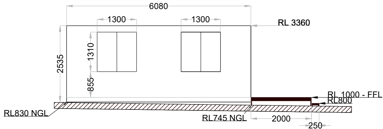
Northern elevation
