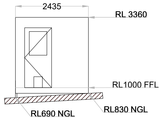
Western elevation
