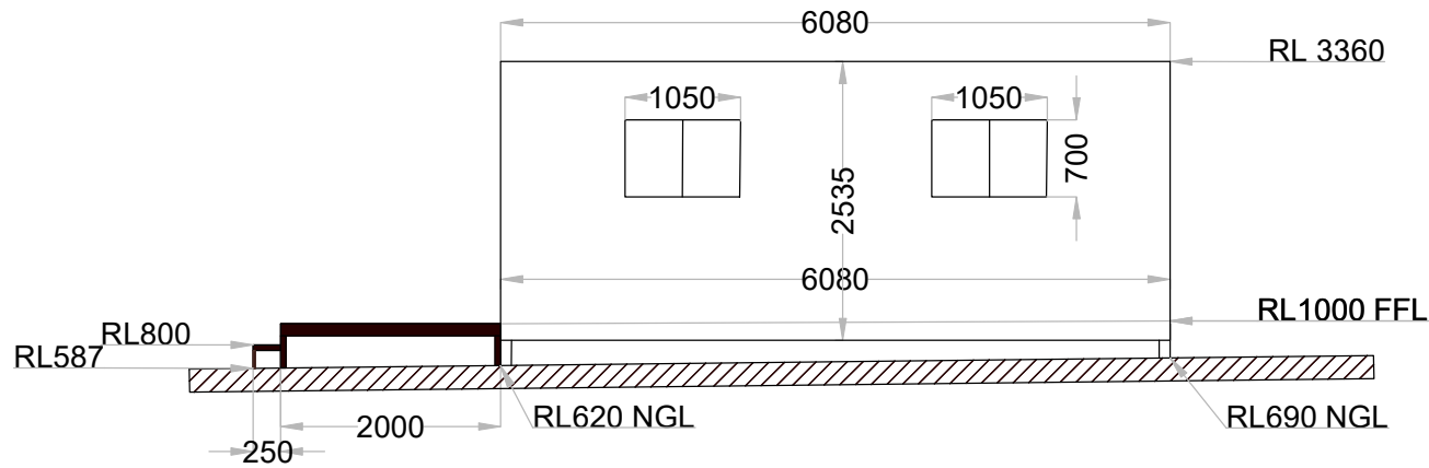
Southern Elevation
