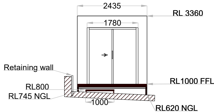
Eastern elevation
