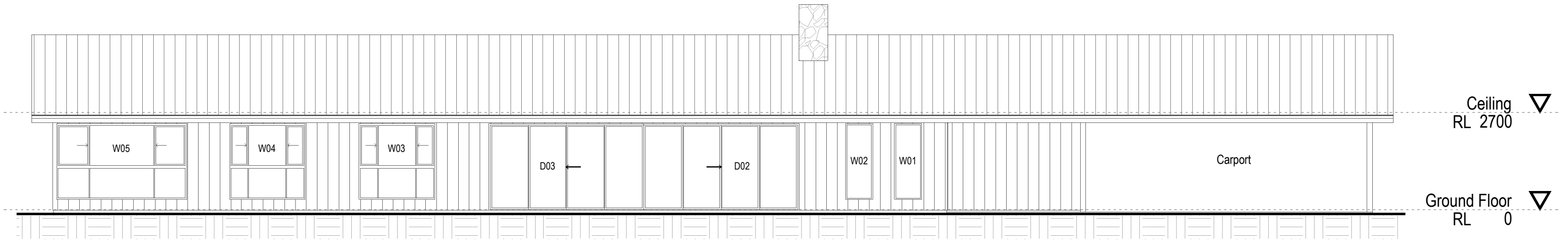
3 North Elevation 1 : 100
