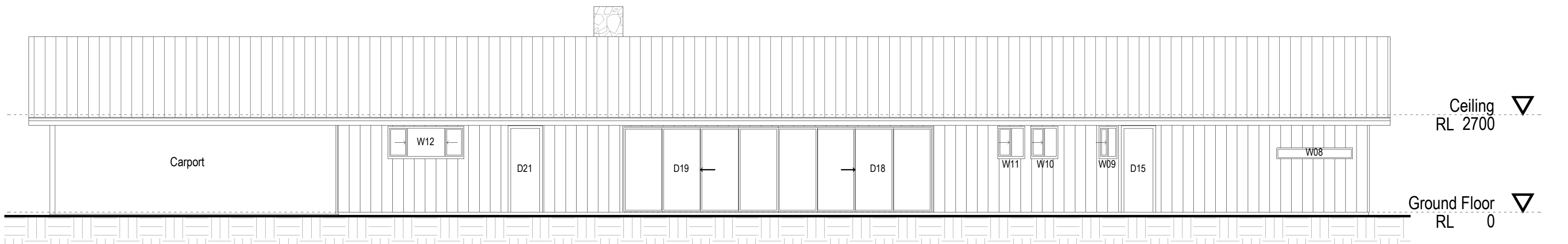
4 South Elevation 1 : 100
