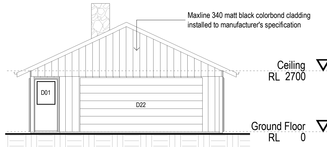
6 West Elevation 1 : 100
