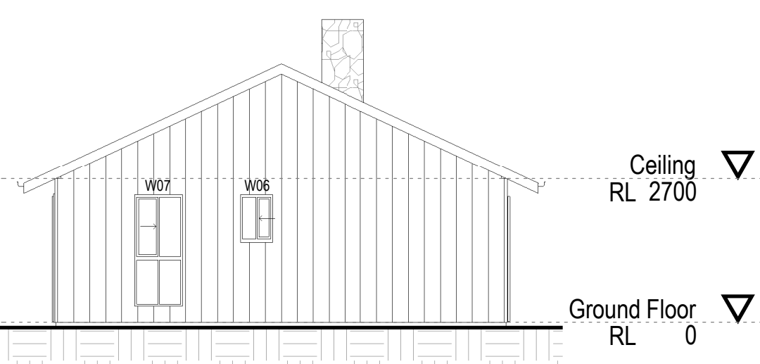
5 East Elevation 1 : 100
