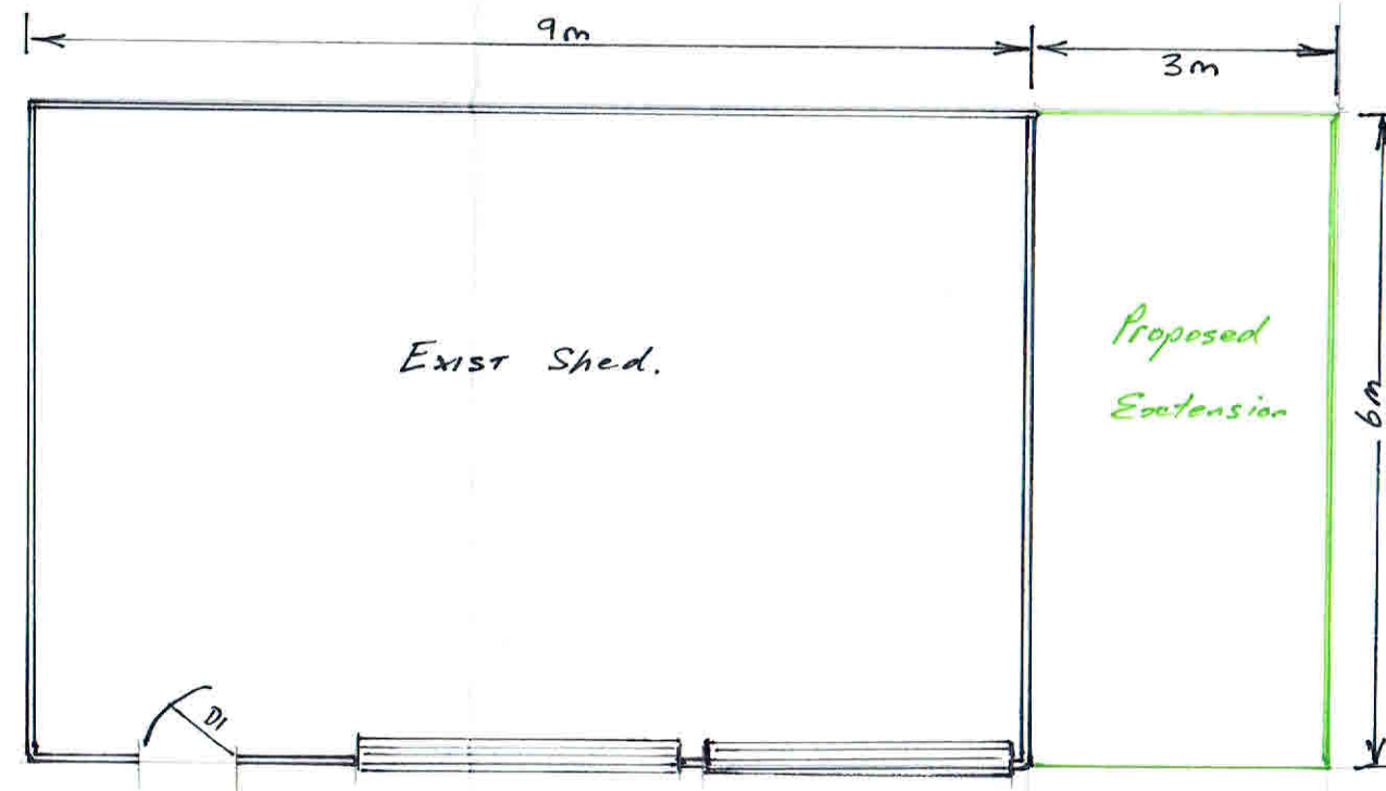
FLOOR PLAN
