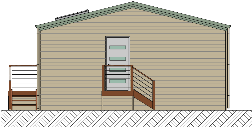
E-04 south west elevation 1:70
