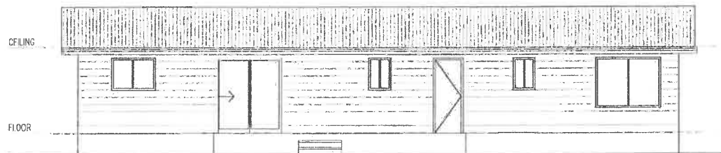
NORTH ELEVATION
