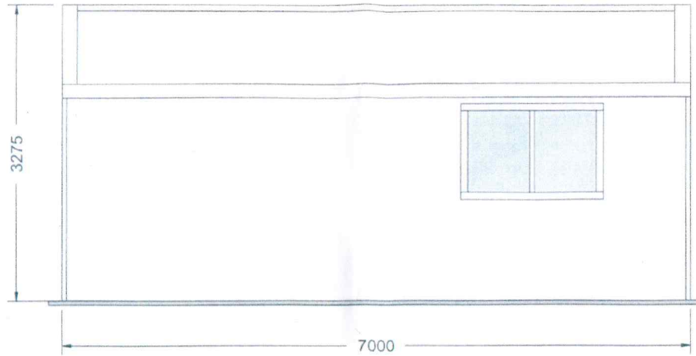
LEFT ELEVATION
