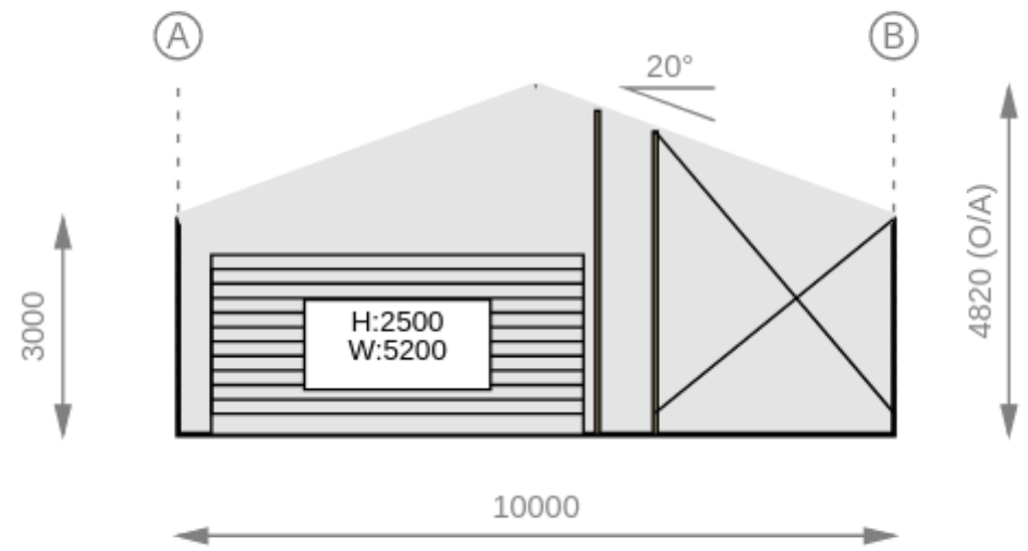
SOUTH WALL
