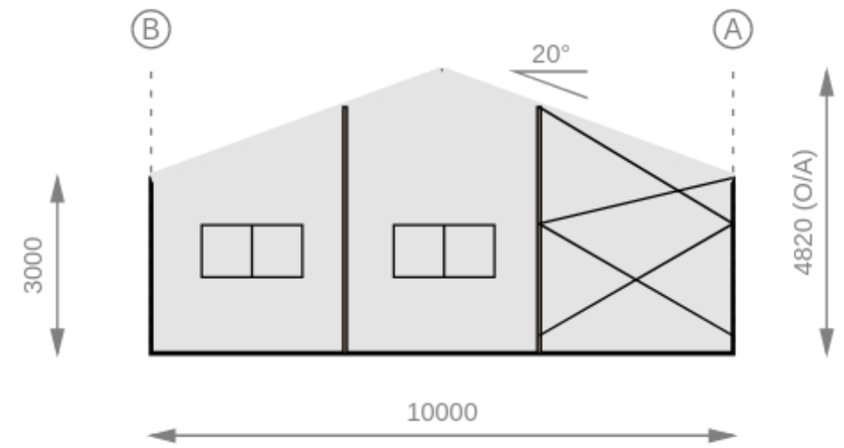
NORTH WALL
