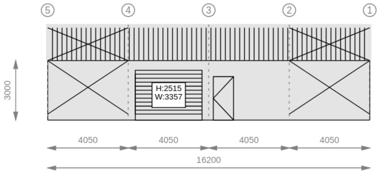
WEST WALL
