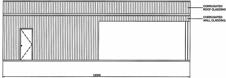
1 6 SIDEWALL EXTERIOR ELEVATION SCALE: 1 = 100
