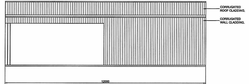
2 6 SIDEWALL EXTERIOR ELEVATION SCALE: 1 = 100
